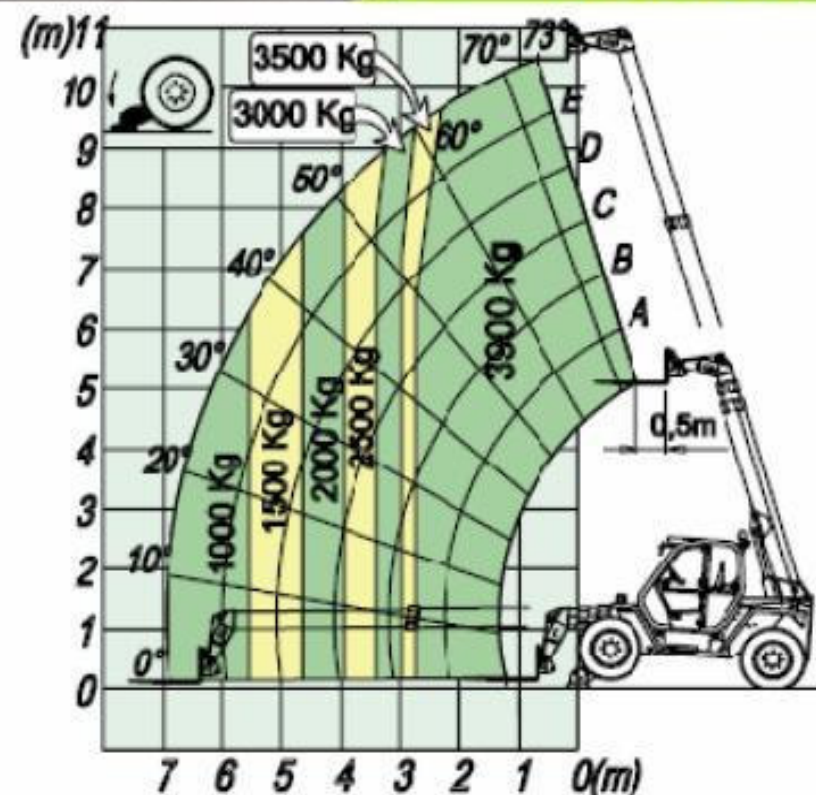
MERLO P39.10
